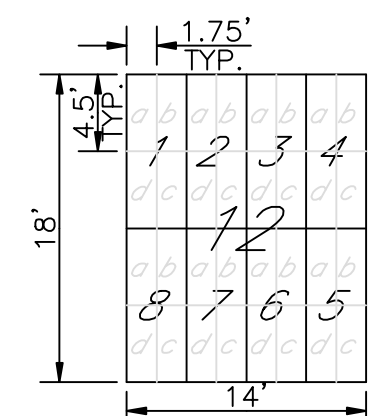
TYPICAL SPACE NUMBERING LOTS 4 & 12, BLOCK "B"
